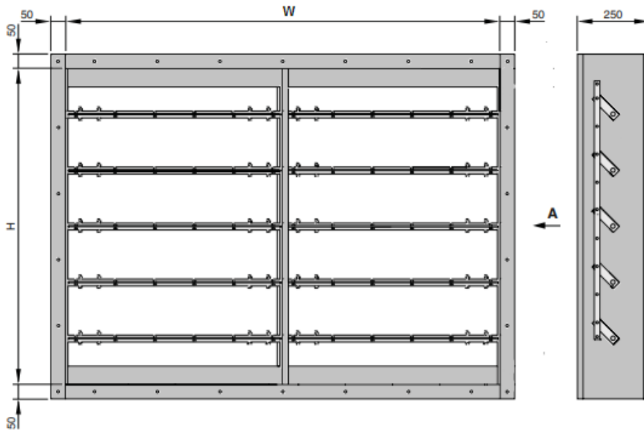
Parallel Blades
