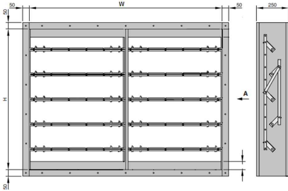
Opposed Blades
