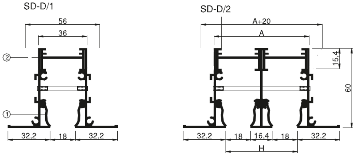
① Air supply direction blade ② Volume damper
