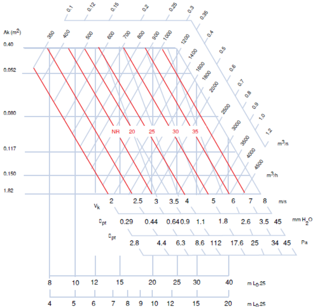
SUPPLY - SELECTION DIAGRAM
