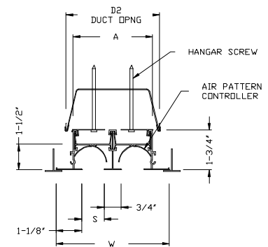
T-BAR (-6 MOUNTING)
