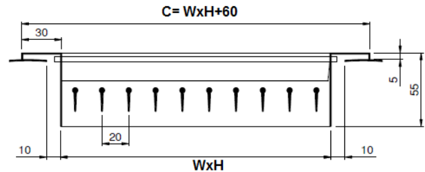
YKM-DD TYPE WITHOUT DAMPER
