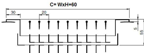
YKM-TD TYPE INCLINED HIT WITH DAMPER
