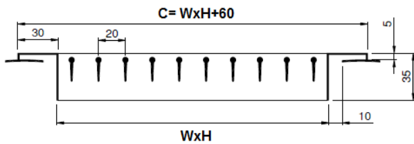
YKM-TD TYPE WITHOUT DAMPER
