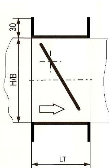
Duct form "D"
