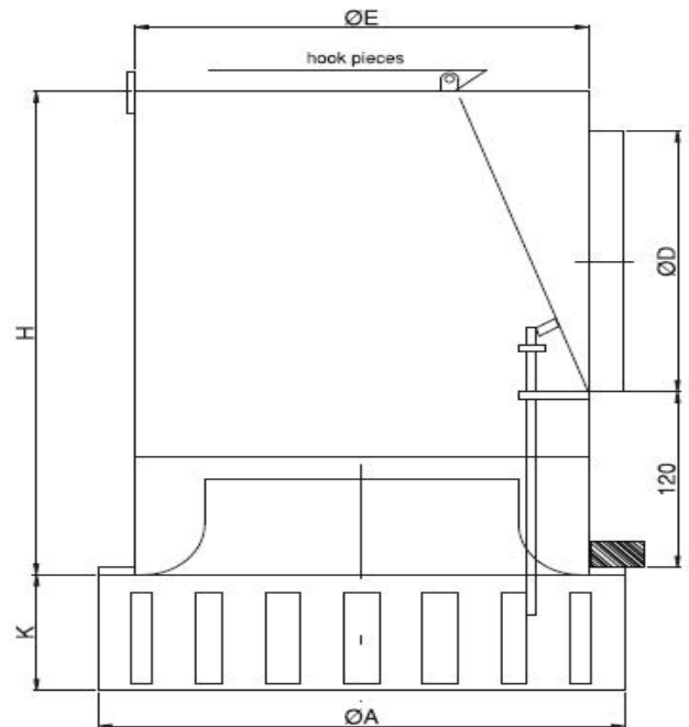
IKD-PL Type With Plenum Box
