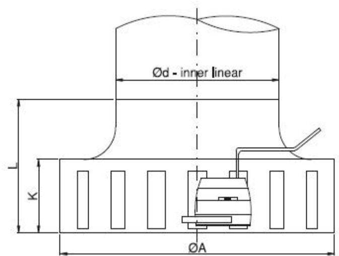
IKD-M Type With Electric Motor
