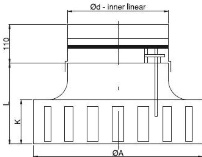
IKD-AY Type Adjustable Neck
