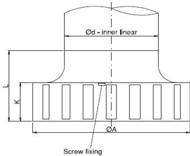
IKD-S Standard Type
