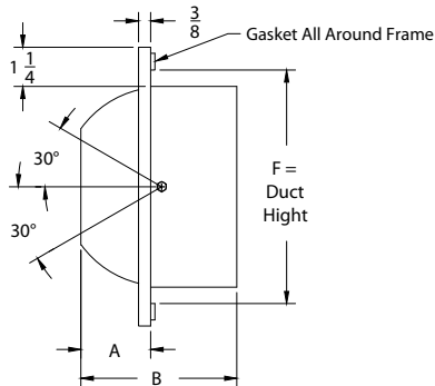
Model: RL-GO (Roto Louver - With Gang Operator)
