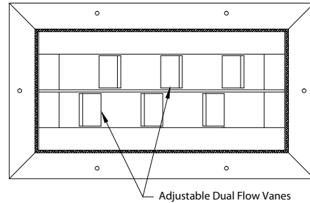
Model: RL-DF (Roto Louver - Dual Flow Blades)
