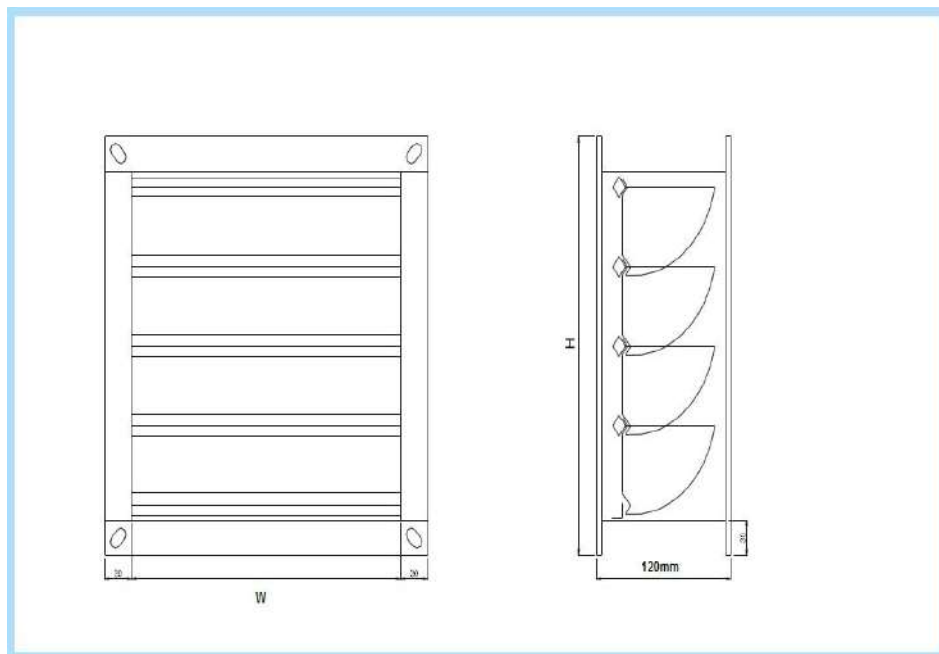
BDD-1 Rectangular Back Draft Damper
