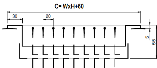
YKM-TD TYPE INCLINED HIT WITH DAMPER
