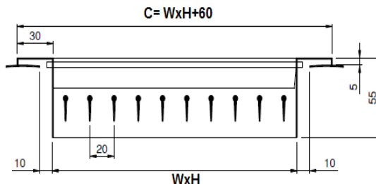
YKM-DD TYPE WITHOUT DAMPER
