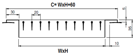
YKM-TD TYPE WITHOUT DAMPER
