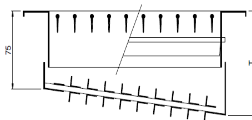
YKM-DD TYPE INCLINED HIT WITH DAMPER
