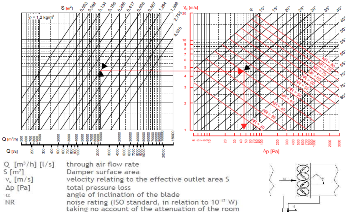
VCD-PRESSURE DROP AND NOISE LEVELS
