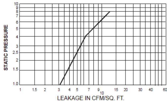
LEAKAGE DAMPER SIZE 36 x 48
